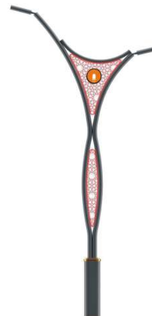
PRODUCT CODE 1752 - DNA POWER 30W, 50W, 100W CCT 3000K, 6000K MATERIAL TYPE M.S / ALUMINIUM POWDER COATED HEIGHT 10FT 12FT 15FT MRP
