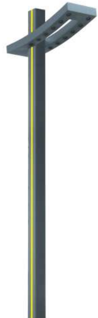
PRODUCT CODE 1729 - OBLONG PRO POWER 30W, 50W, 100W CCT 3000K, 6000K MATERIAL TYPE M.S / ALUMINIUM POWDER COATED HEIGHT 10FT 12FT 15FT MRP
