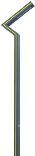
PRODUCT CODE 1720 - ZETA PRO POWER 30W, 50W, 100W CCT 3000K, 6000K MATERIAL TYPE M.S / ALUMINIUM POWDER COATED HEIGHT 10FT 12FT 15FT MRP
